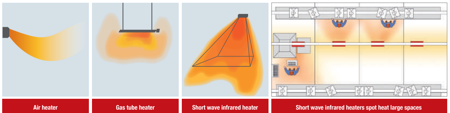
Graphics above demonstrate heating effectiveness in large open indoor areas.
